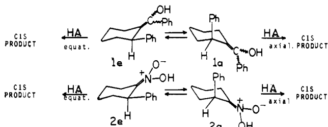
Chart I. cis -1-Benzoyl-2-phenylcyclohexane and cis -1-Nitro-2-phenylcyclohexane Formation
